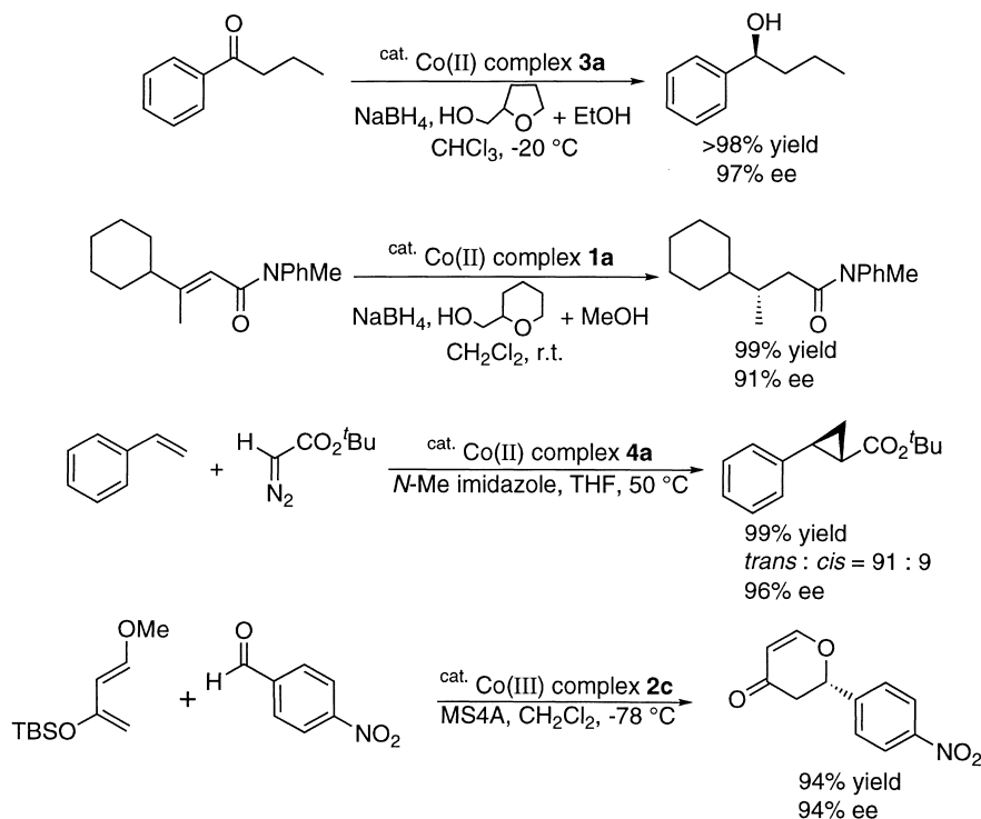
Scheme 1. Enantioselective reactions catalyzed by 3-oxobutylideneaminato complexes.
