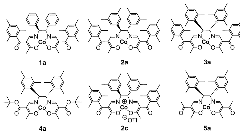
Fig. 1. Varieties of 3-oxobutylideneaminatocobalt complex catalysts.
