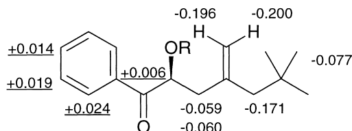
Fig. 2. \Delta\delta(\delta_S - \delta_R) values (ppm) obtained for ( R )- and ( S )-MTPA esters of secondary alcohols.
