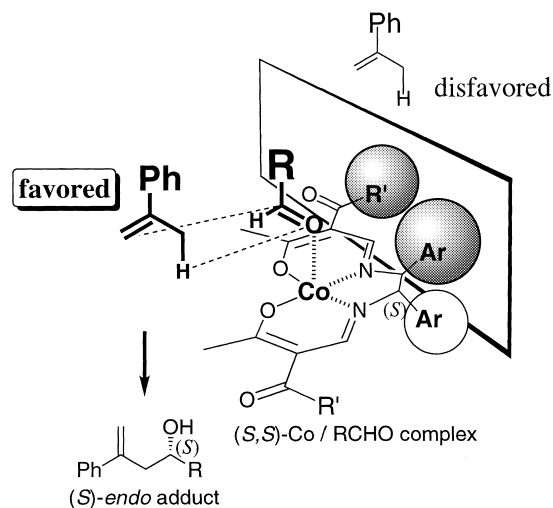
Fig. 3. Reasonable explanation for the enantioselection in the carbonyl-ene reaction catalyzed by the ( S,S )-cobalt complex.
